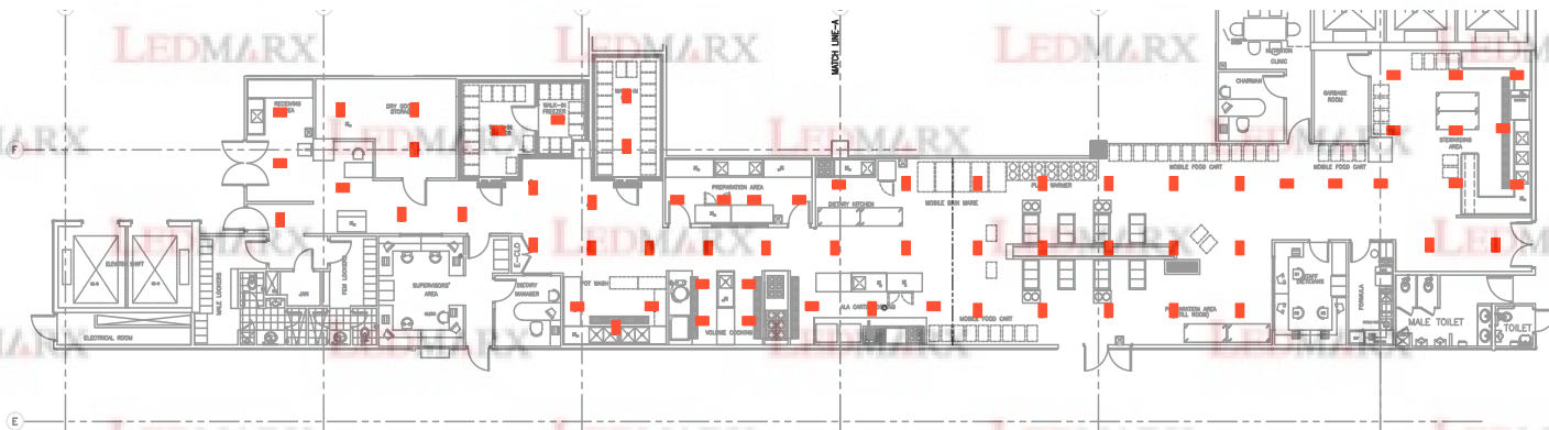
PROPOSED LIGHTING FIXTURE LAYOUT
